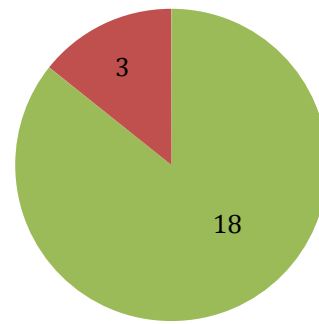
Lurking
