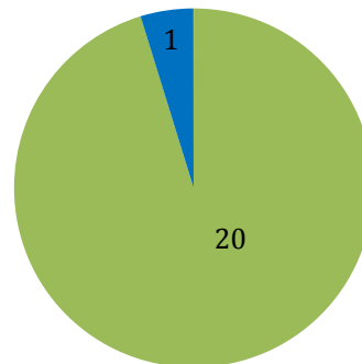
Pseudo-buy/delivery
