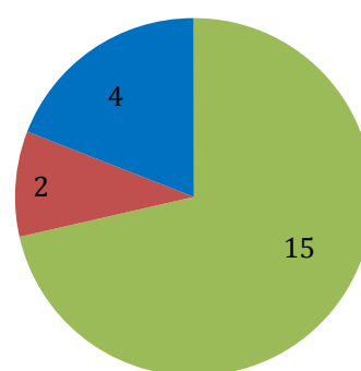
Scraping
